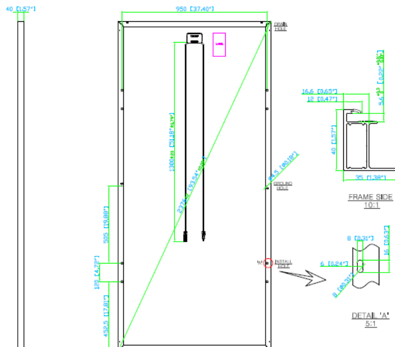
Figure 1.20 – Drawing HSxxxUE-AN1 (2155 X 1000 X 40) (6*13, 78cell module)
