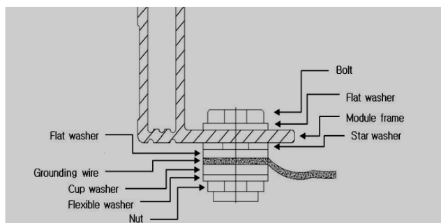
Figure 2 – Grounding method
