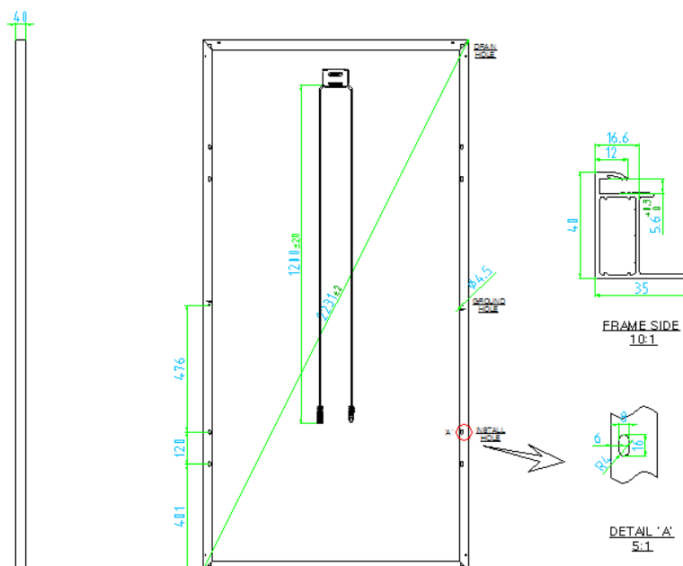
Figure 1.16 – Drawing HSxxxUD-AN1 (1994 X 1000 X 40) (6*12, 72cell module)
