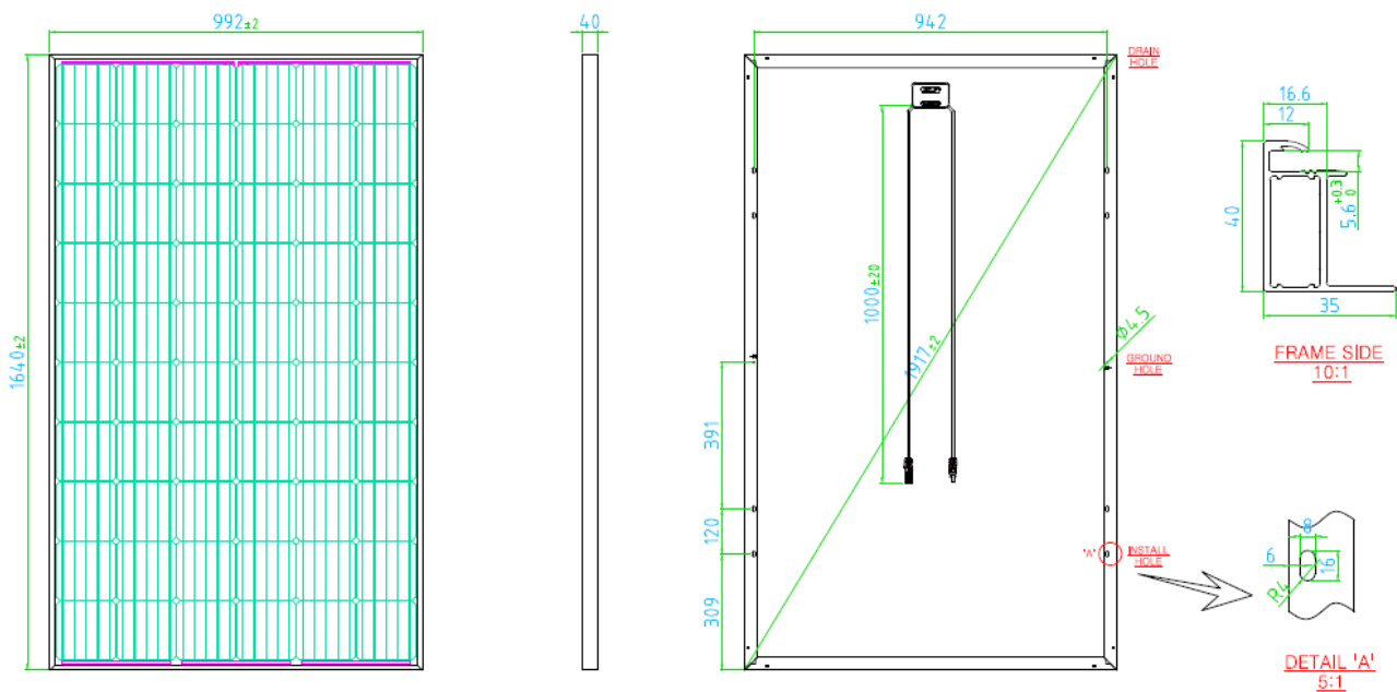
Figure 1.6 – Drawing HSxxxUB-AN1 (1640 X 992 X 40) (6*10, 60cell module)
