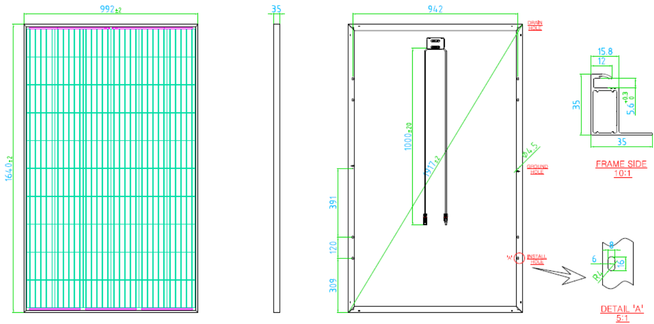
Figure 1.3 – Drawing HSxxxPB-AN1 (1640 X 992 X 35) (6*10, 60cell module)
