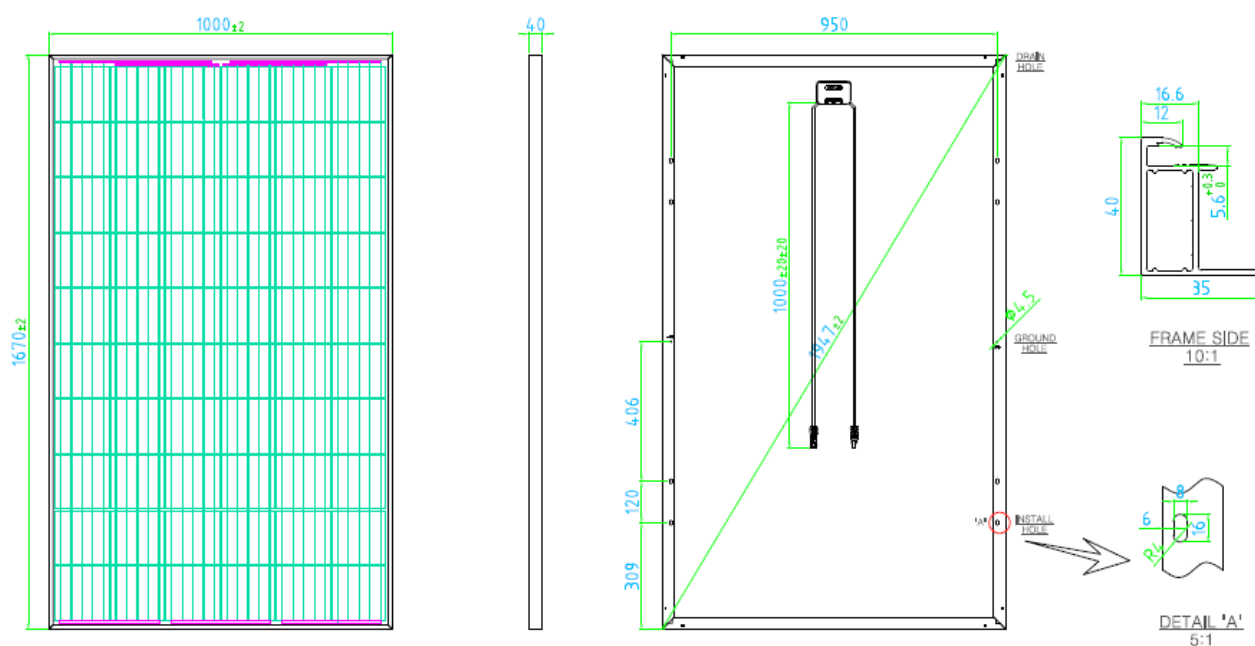
Figure 1.9 – Drawing
