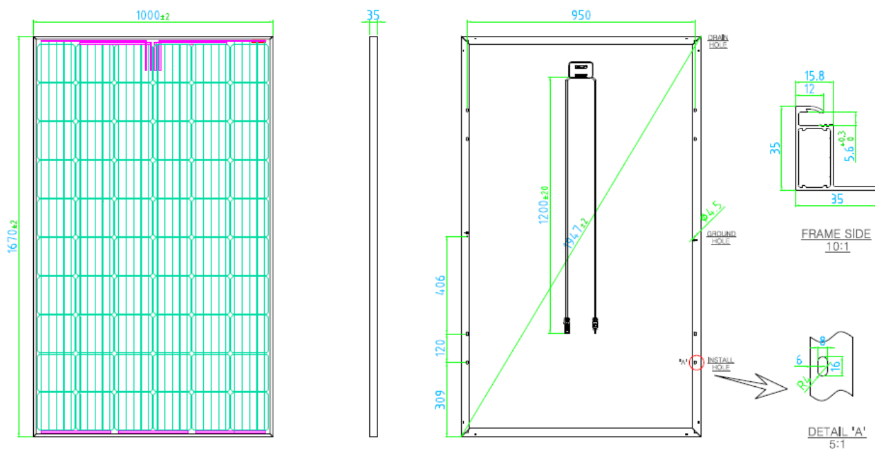
Figure 1.8 – Drawing
