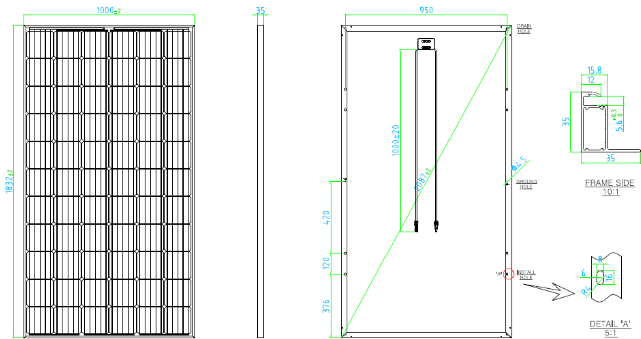
Figure 1.12 – Drawing
