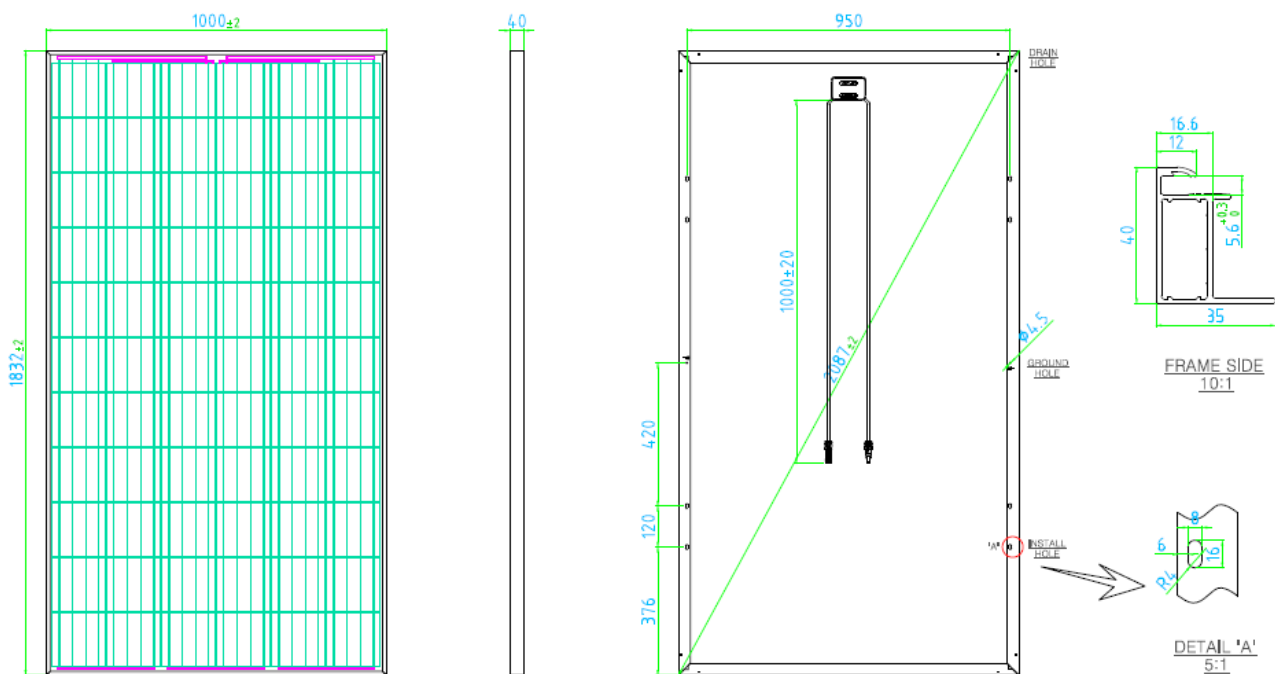
Figure 1.13 – Drawing
